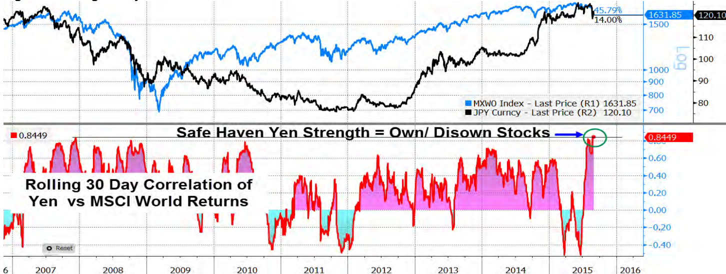
Figure 3: Rolling 30-Day Correlation of the Safe-Haven Yen and MSCI World
